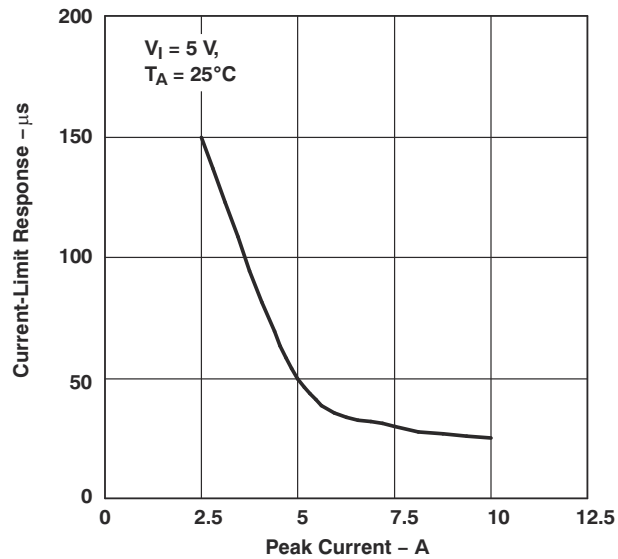
Figure 5-11. Current-Limit Response vs Peak Current
