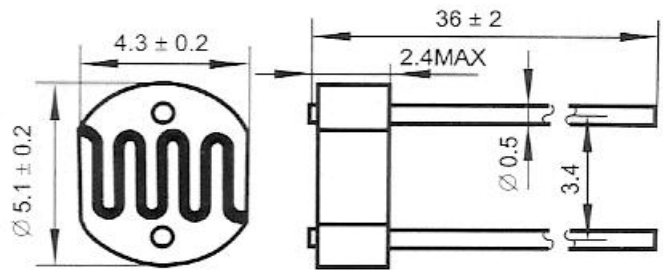
Overall dimension drawing (unit: mm)
